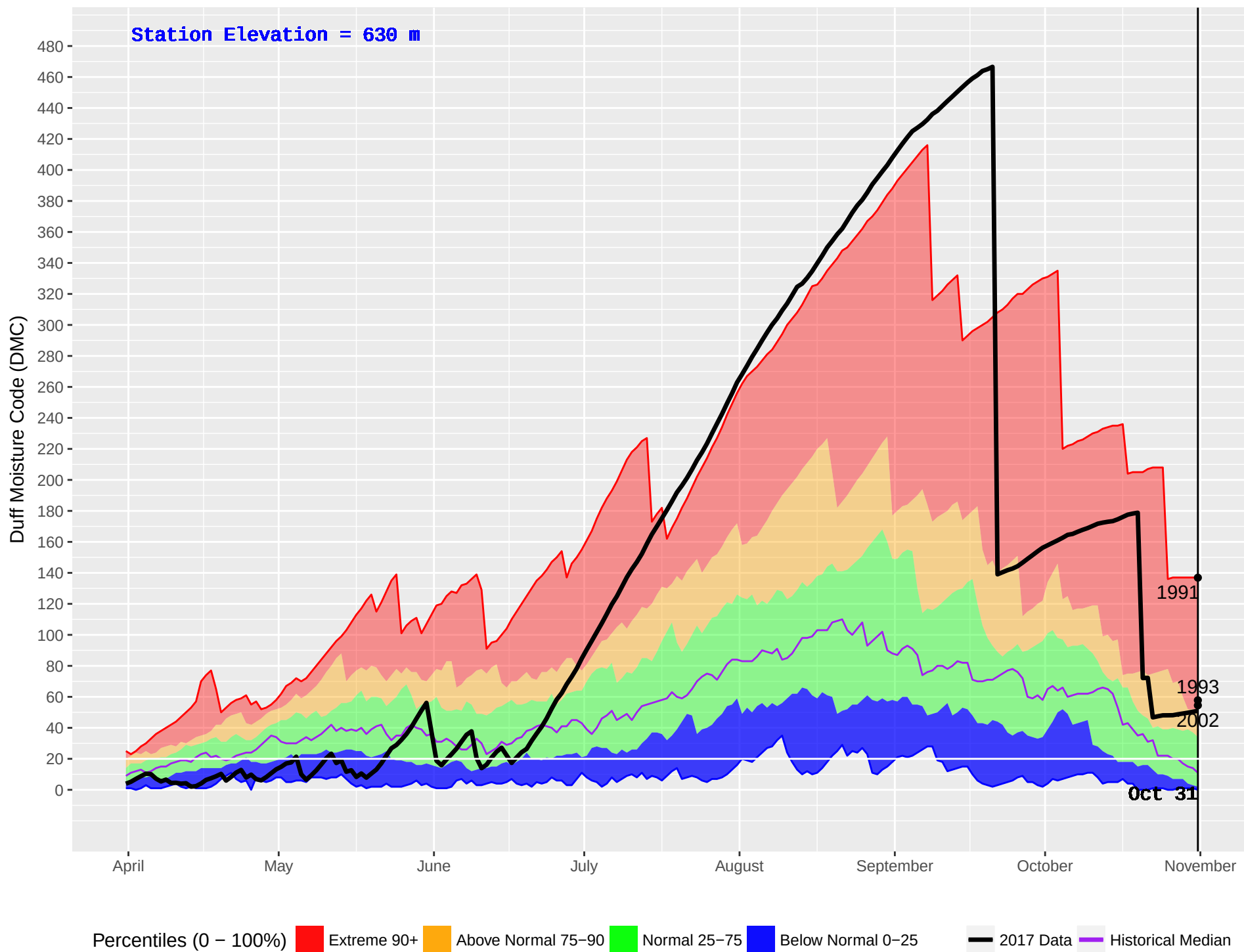
GRAND FORKS (392) : Historical (1981–2016) and Current (2017) Noon Duff Moisture Code (DMC)
