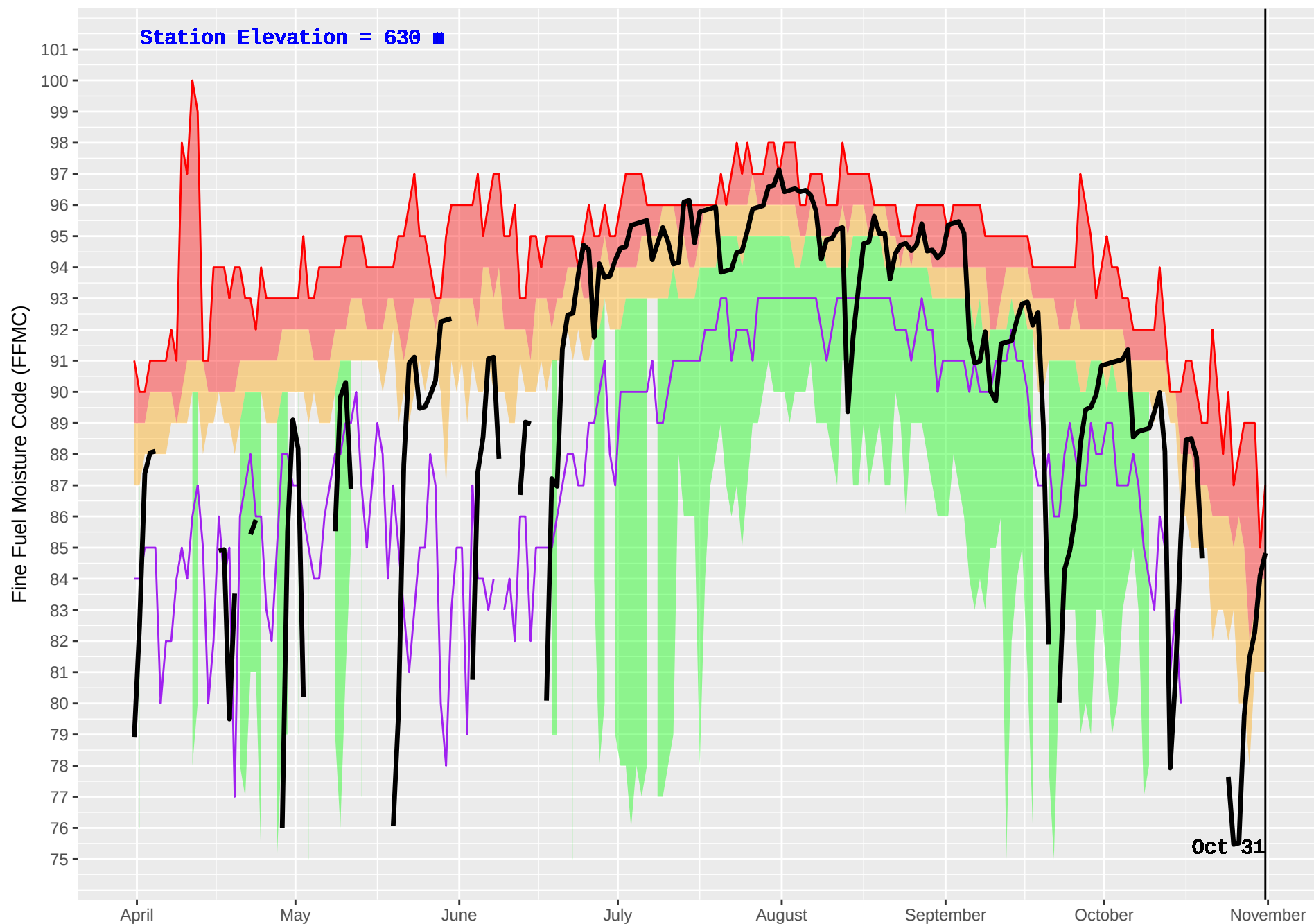
GRAND FORKS (392) : Historical (1981–2016) and Current (2017) Noon Fine Fuel Moisture Code (FFMC)
